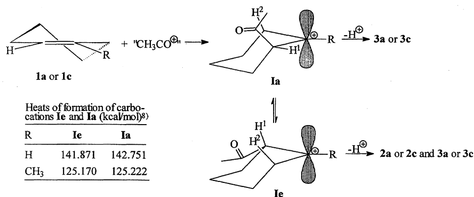
Scheme 3. Formation of 2-acetylcyclohexyl ( \text{R}=\text{H} ) and 2-acetyl-1-methylcyclohexyl cations ( \text{R}=\text{CH}_3 ) and production of the corresponding ketones.
